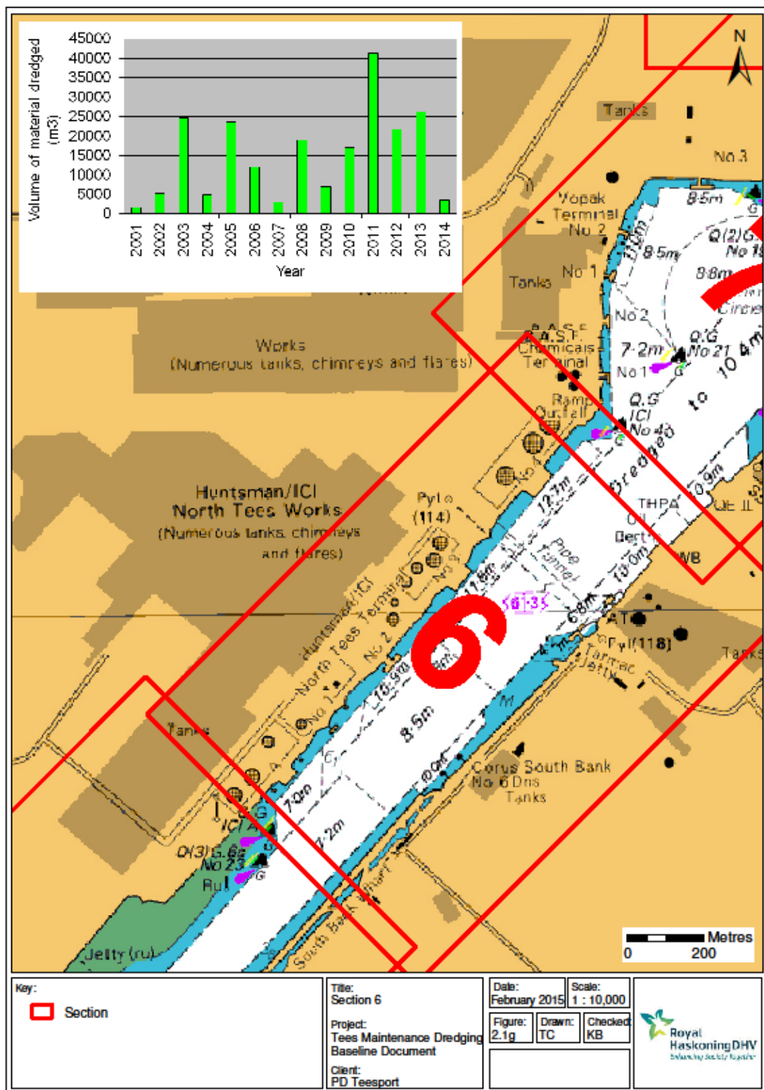
Figure 2.1g The volume of maintenance dredged material (m³) in reach 6 during the period 2001 – 2014
