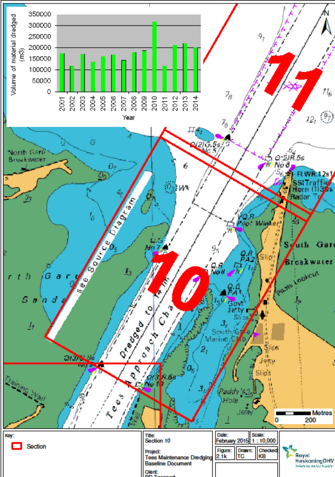
Figure 2.1k The volume of maintenance dredged material (m 3 ) in reach 10 during the period 2001 – 2014
